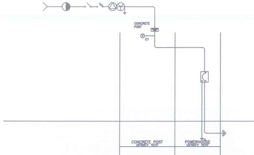
POWER SYSTEM RISER DIAGRAM SCALE: 1/2" = 1'-0" NTS
